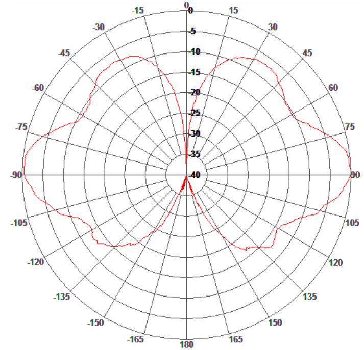
E-Plane Pattern
