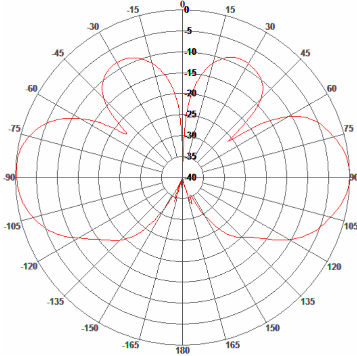
E-Plane Patterns
